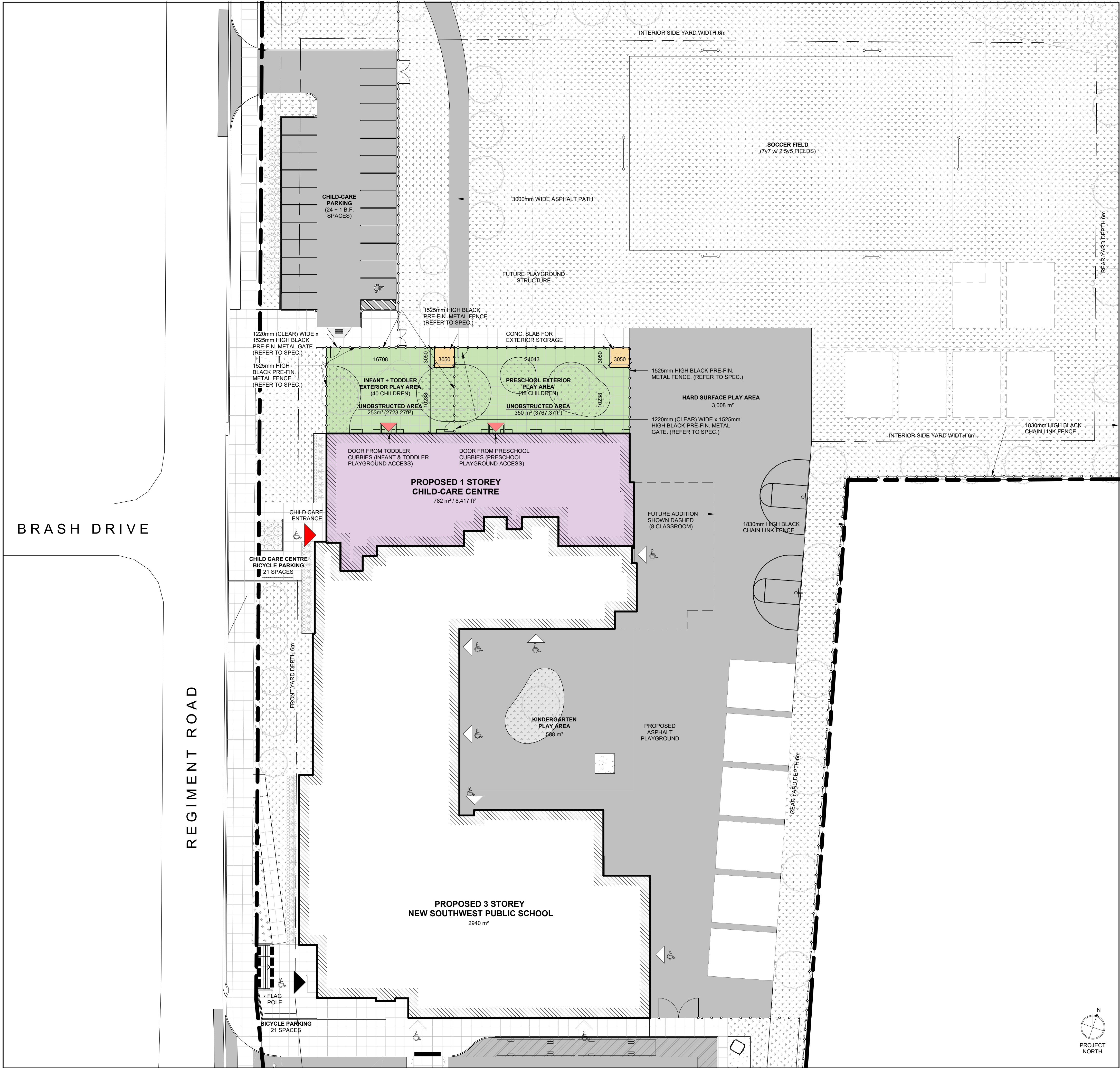
1 SITE PLAN - CHILD CARE CENTRE CC1.01 0 5 10 20 30 m 1:300
